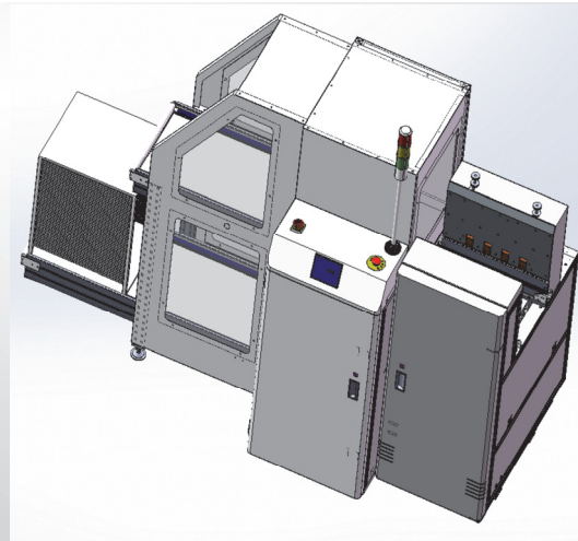
Loader/Destacker Combo
