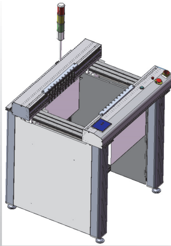
Reject Conveyor
